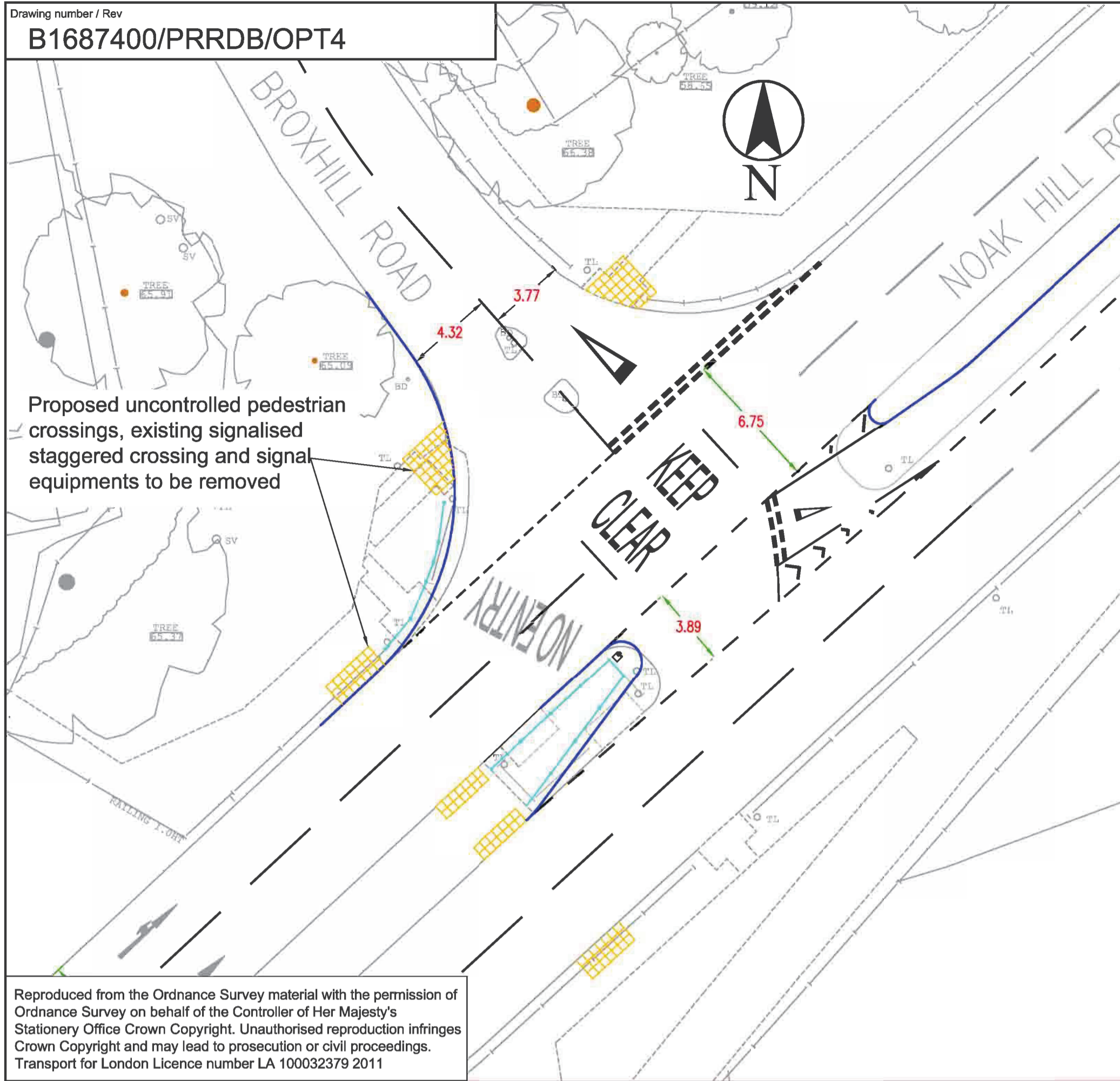
SIGNAL LAYOUT SCALE 1:200
