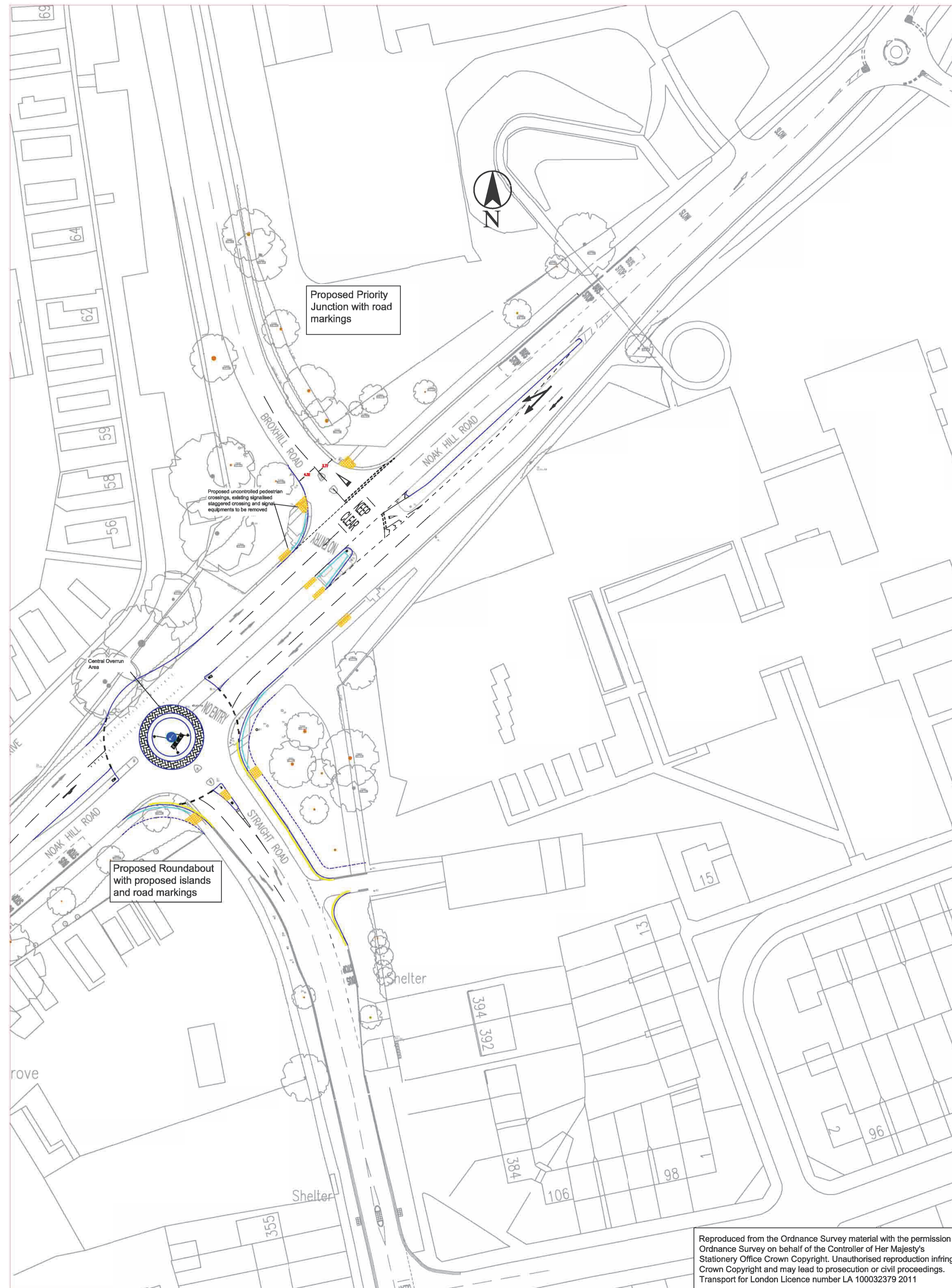
LAYOUT SCALE 1:500
