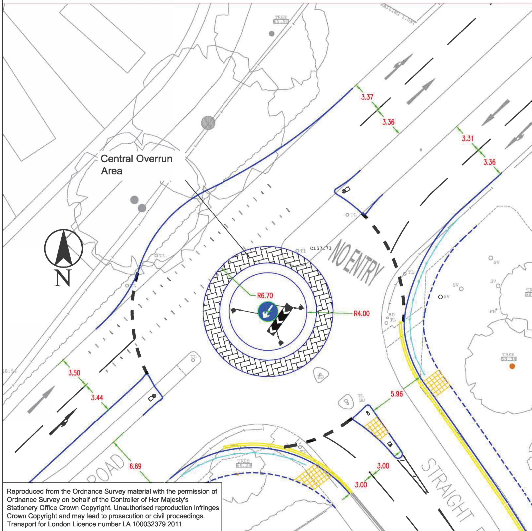
SIGNAL LAYOUT SCALE 1:200
